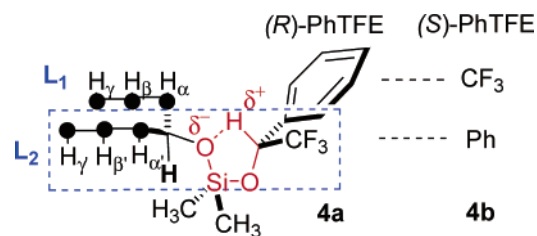
Figure 1. General conformational model for the PhTFE derivatives discussed in the text.
